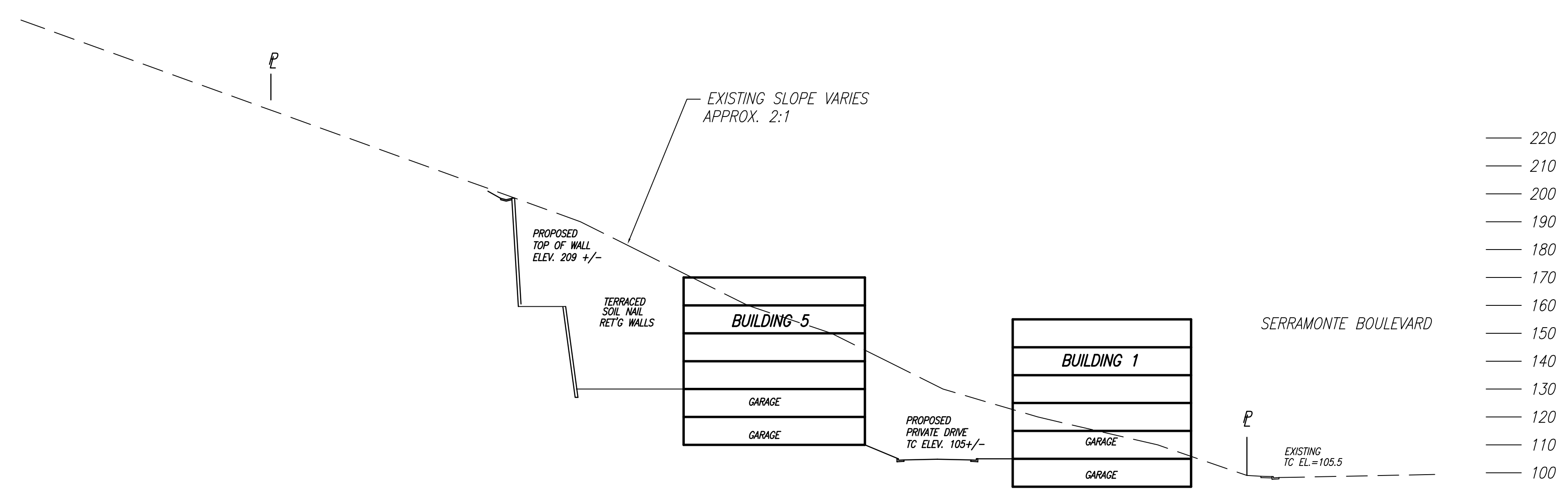
GRAND SECTION THRU BLDG 1 AND 5 FROM SERRAMONTE BLVD. TO RIDGELINE
